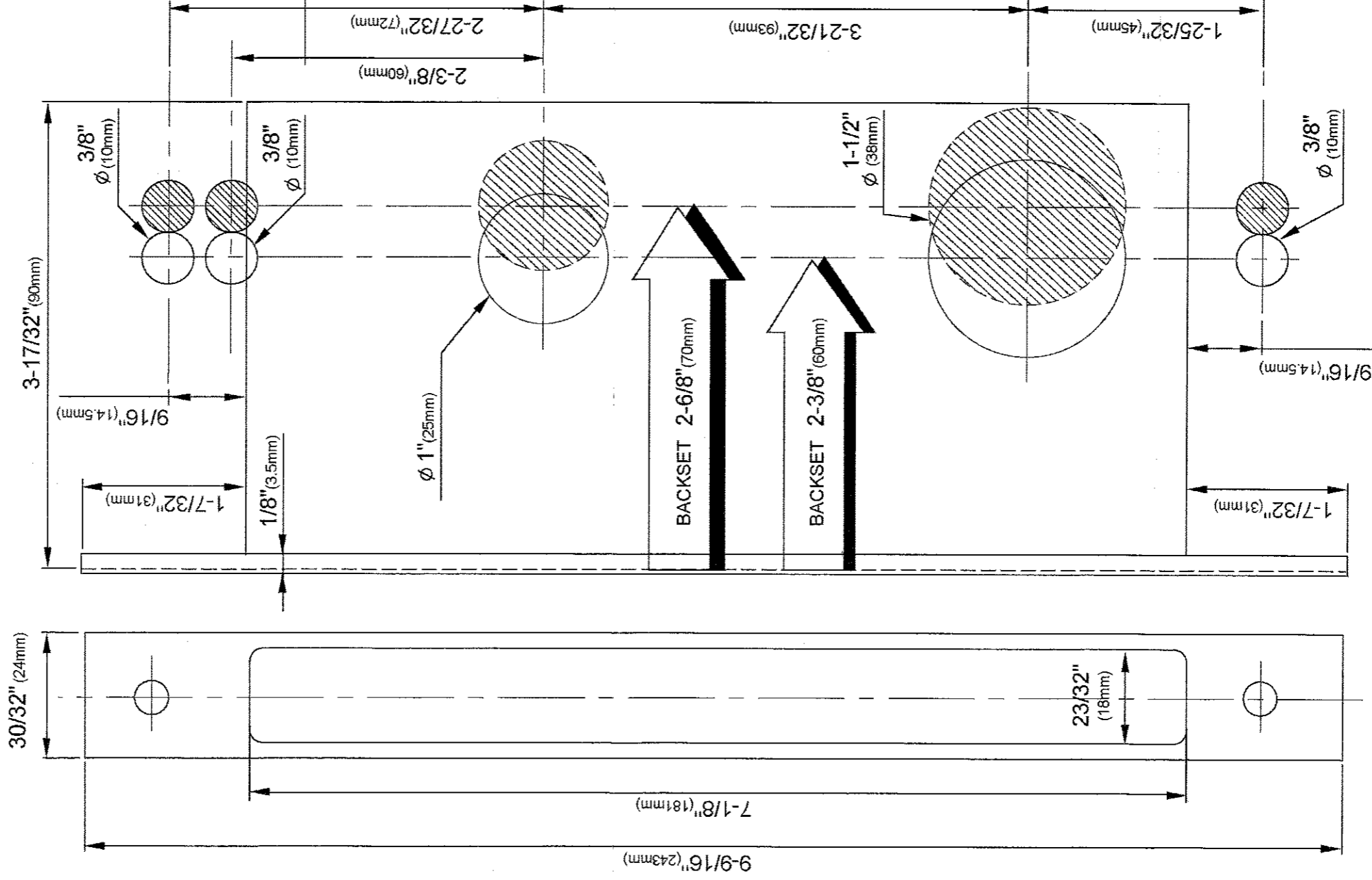
LOCK CASE MORTISE
